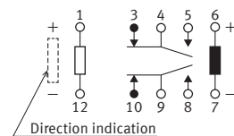
Schematic ( BOTTOM VIEW ) ( Reset ) ( Operation function LT )
