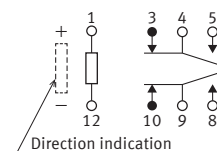
Schematic ( BOTTOM VIEW ) ( De-energize )
