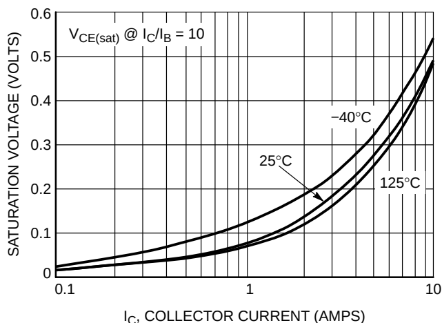
Figure 6. D45VH10 ON-Voltage
