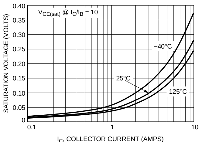
Figure 5. D44VH10 ON-Voltage
