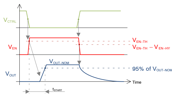
Figure 70. Startup Timing – EN Pin Controlled by Transistor
