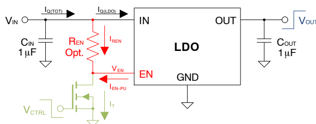
Figure 69. Circuit – EN Pin Controlled by Transistor
