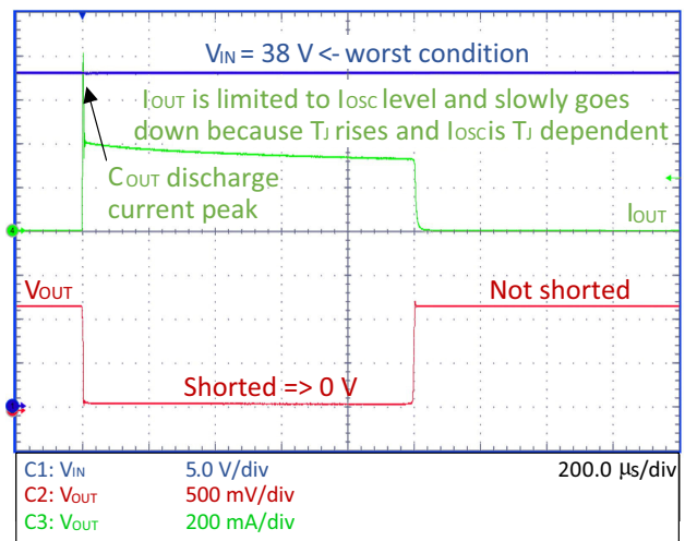
Figure 39. Output Short (1 ms) – NCP730–ADJ–1.2 V
