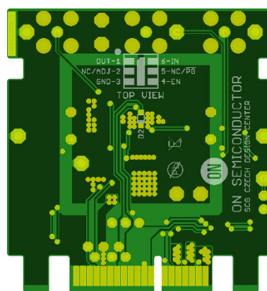
Figure 95. WDFN-6 2x2 Demo Board (2 layer, rev. 1) – PCB Bottom Layer
