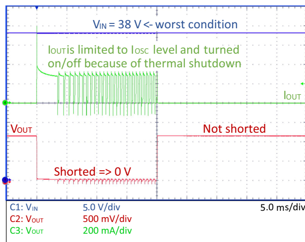
Figure 40. Output Short (20 ms) – NCP730–ADJ–1.2 V
