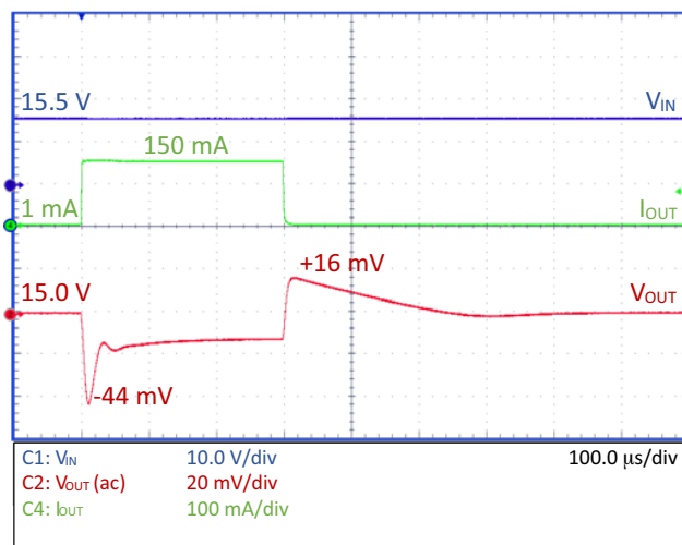
Figure 30. Load Transient – NCP730–15.0 V, C_{OUT} = 50\text{ }\mu\text{F}
