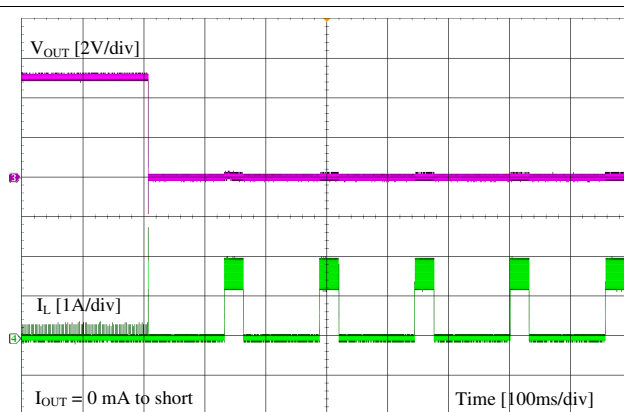
Figure 9-8. Short Protection
