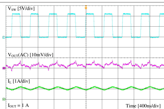
Figure 9-4. Ripple at Full Load
