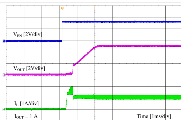
Figure 9-6. Start-Up by EN
