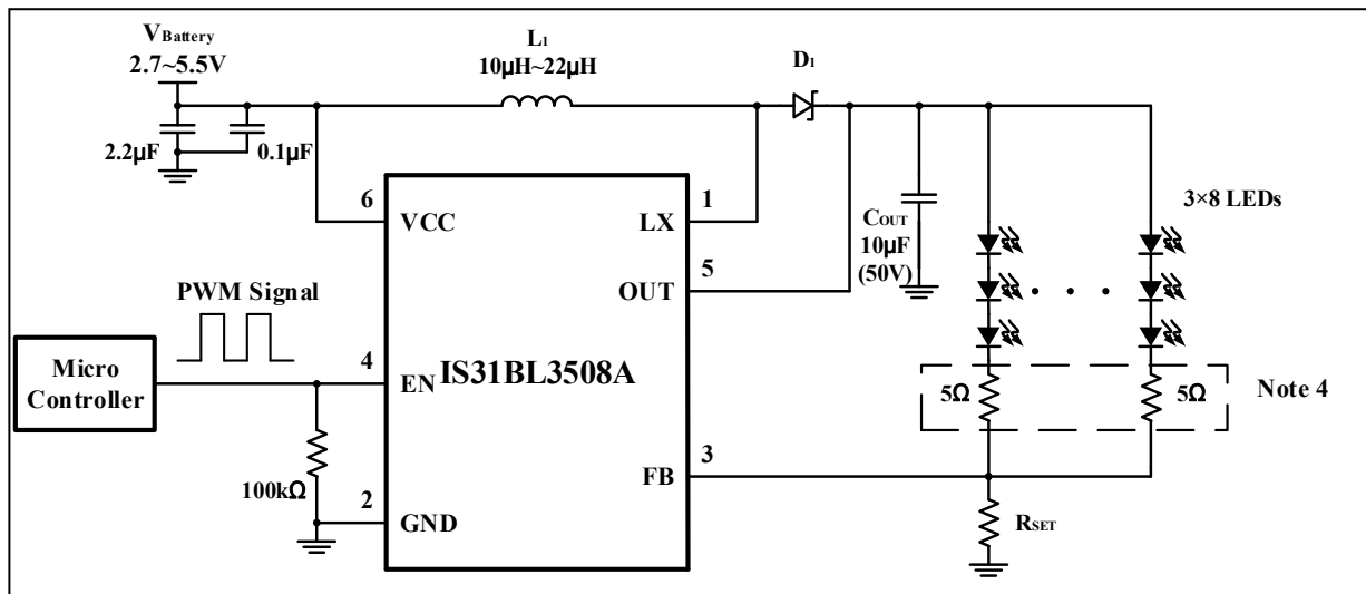
Figure 3 Constant Current White LED Driver Using PWM At The EN Pin To Control Intensity 3×8 LEDs
