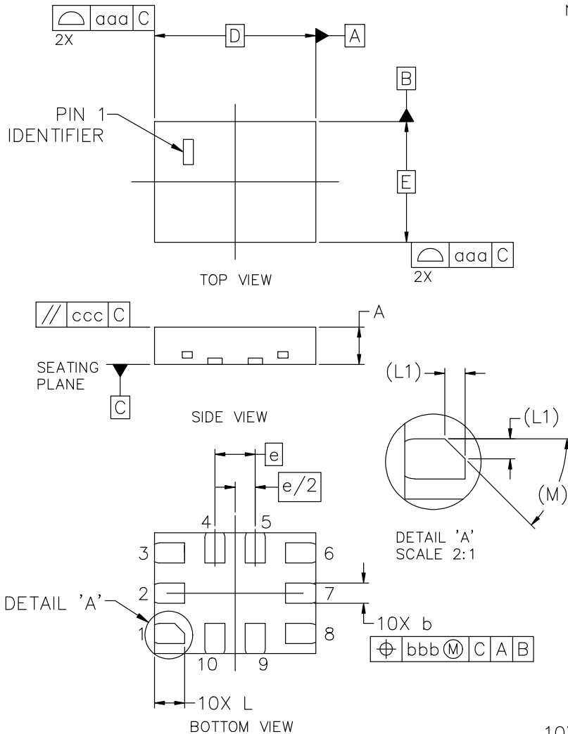
X2QFN-10 1.60x1.20x0.37, 0.40P CASE 722AC ISSUE B
