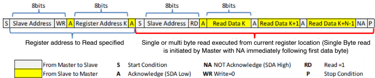
Figure 6. I 2 C Read Example
