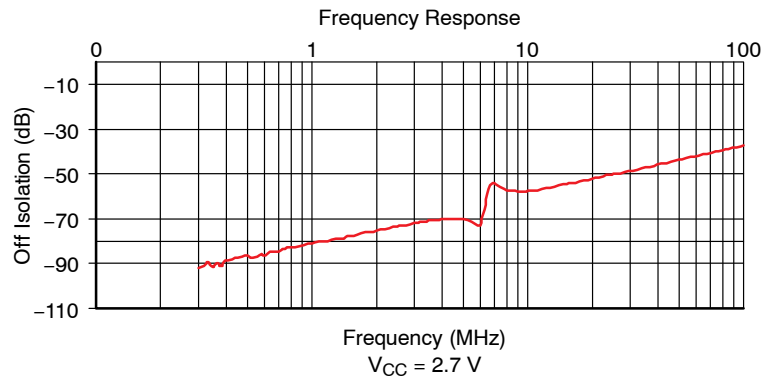
Figure 6. Off Isolation
