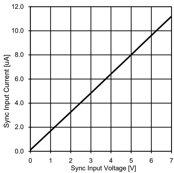
Fig.28 ISYNC-VSYNC
