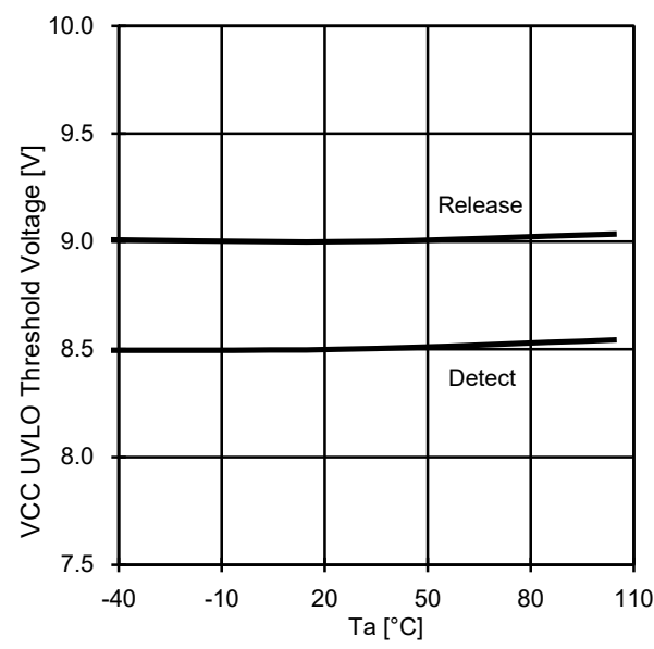
Fig.9 VCC UVLO-Ta
