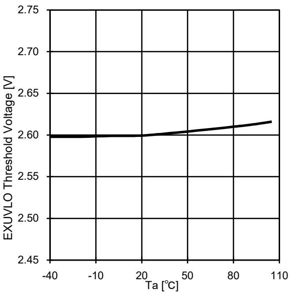
Fig.10 EXUVLO (CTL)-Ta
