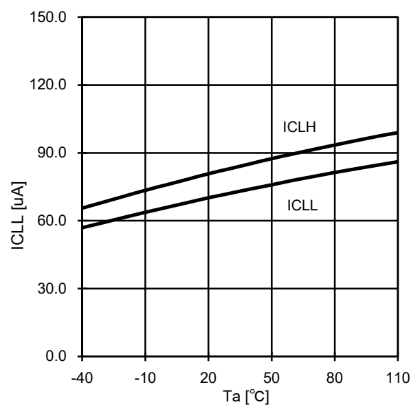
Fig.22 ICLH, ICLL-Ta
