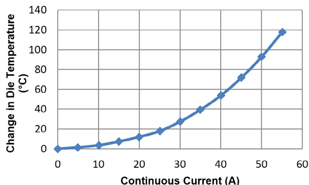
Figure 9: Self Heating in the EX Package Due to Current Flow
