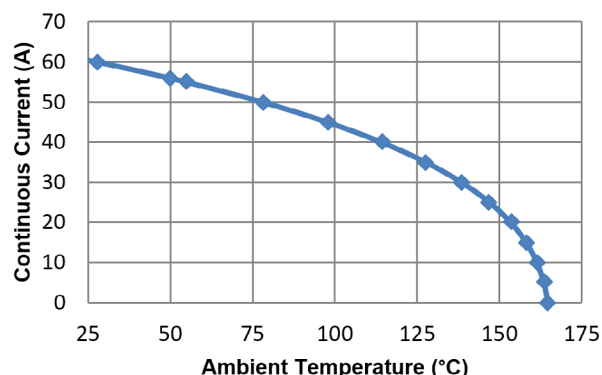
Figure 10: Maximum Continuous Current in the EX package at a Given T_A
