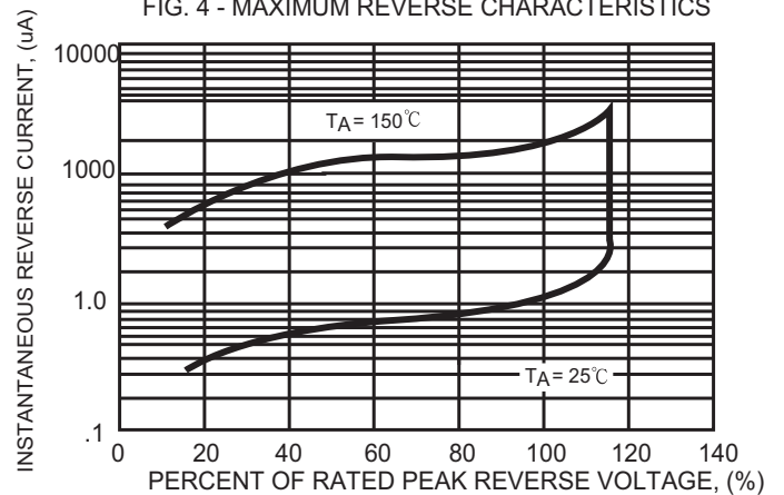
FIG. 4 - MAXIMUM REVERSE CHARACTERISTICS
