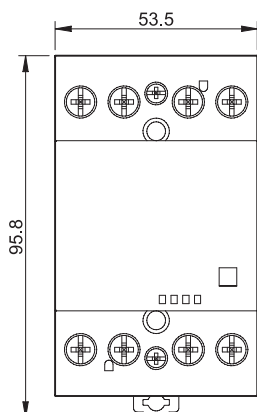
Type 22.72 Box clamp
