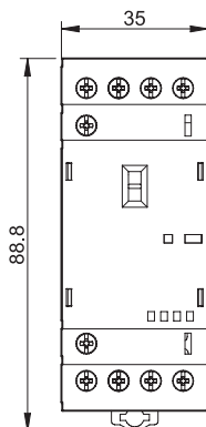
Types 22.44/22.64 + 022.63/022.65 Box clamp
