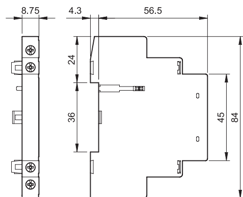
Types 022.73/022.75 Box clamp
